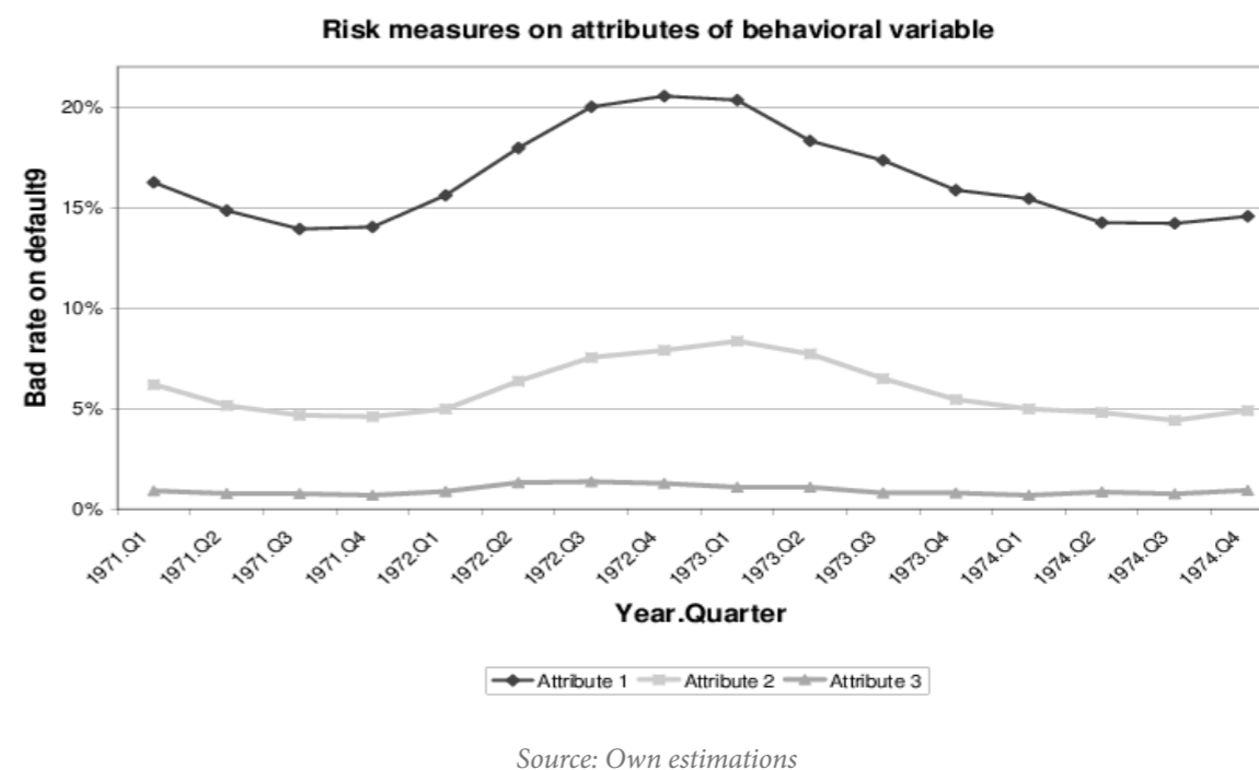
Figure 3: Risk measures on Default t , on attributes of a variable x_{n_{due}}^{beh}(6) for the case APP
