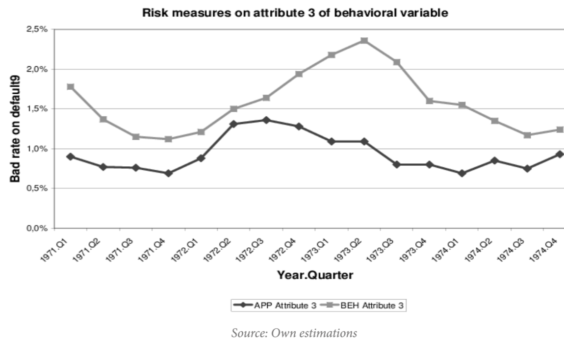
Figure 2: Risk measures on Default t , on attribute 3 of a variable x_{n_{due}}^{beh}(6) for two cases APP and BEH
