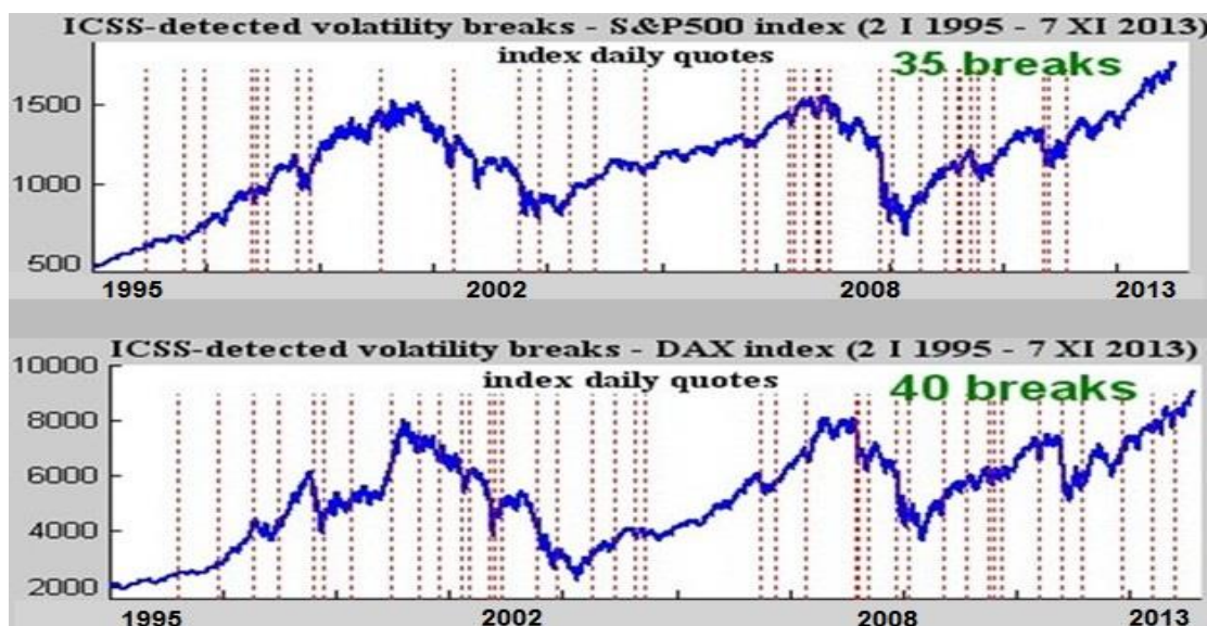
Figure 5: Detection of structural breaks in S&P500 and DAX30 indices: ICSS algorithm
