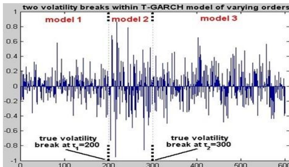
Figure 4: Simulated path of T-GARCH model (11), T=600, with 2 breaks at \tau_1=200 , \tau_2=300
