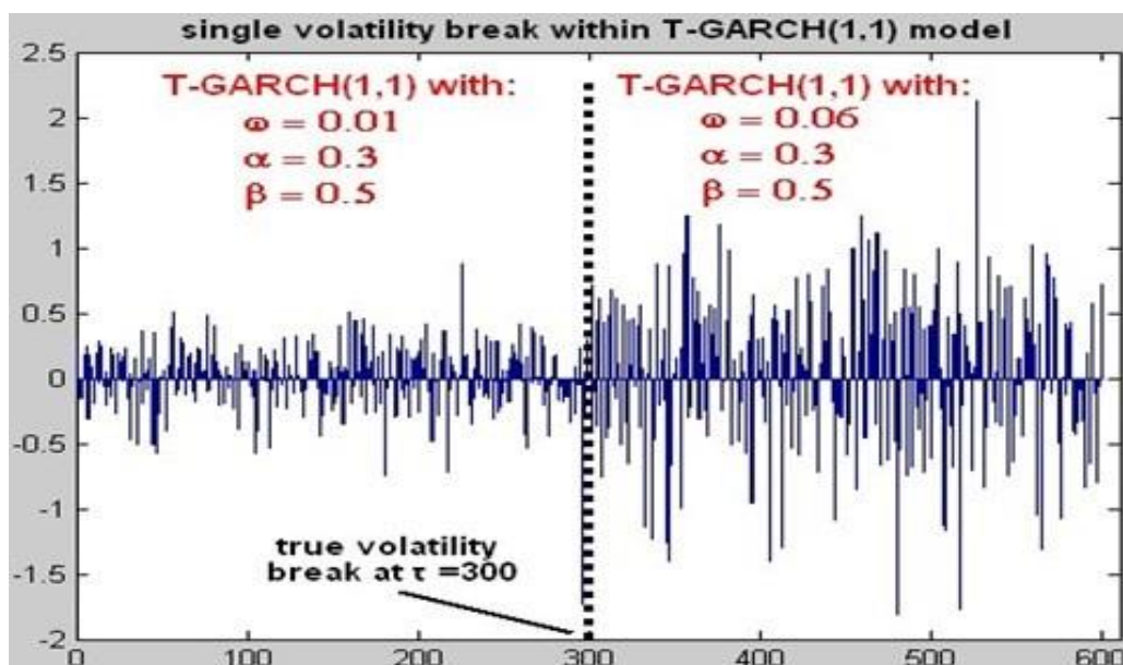
Figure 3: Simulated path of T-GARCH(1,1) model (9), T=600 , with single volatility break at \tau=300
