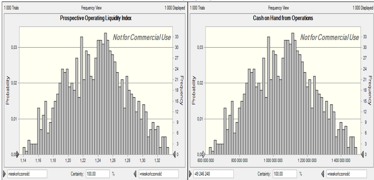
Figure 2. Simulated distribution of Prospective Operating Liquidity Index and cash on hand from operations of Jeronimo Martins Dystrybcja S.A. for 2014
